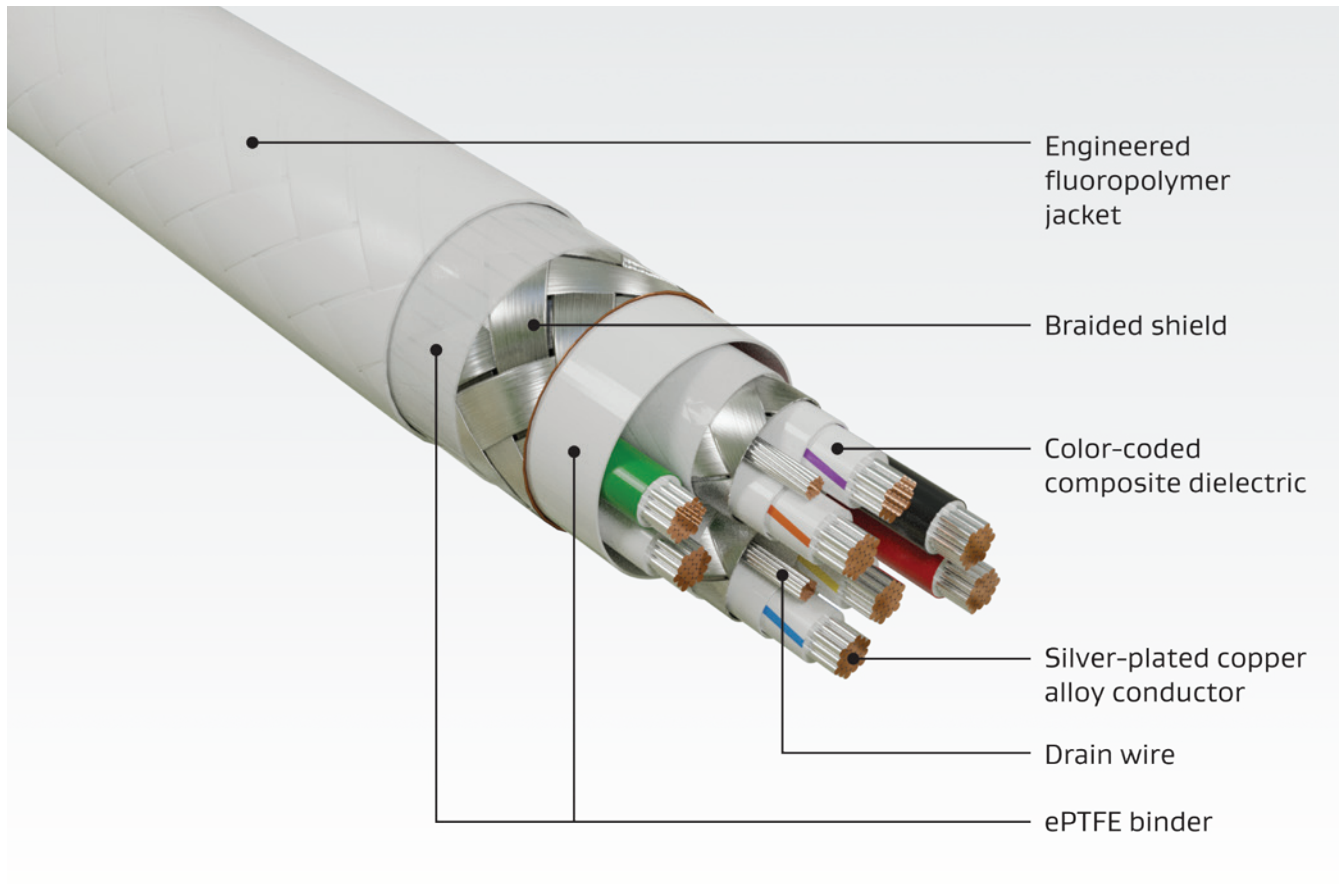
Figure 32: Sturdy Cable Bundle
