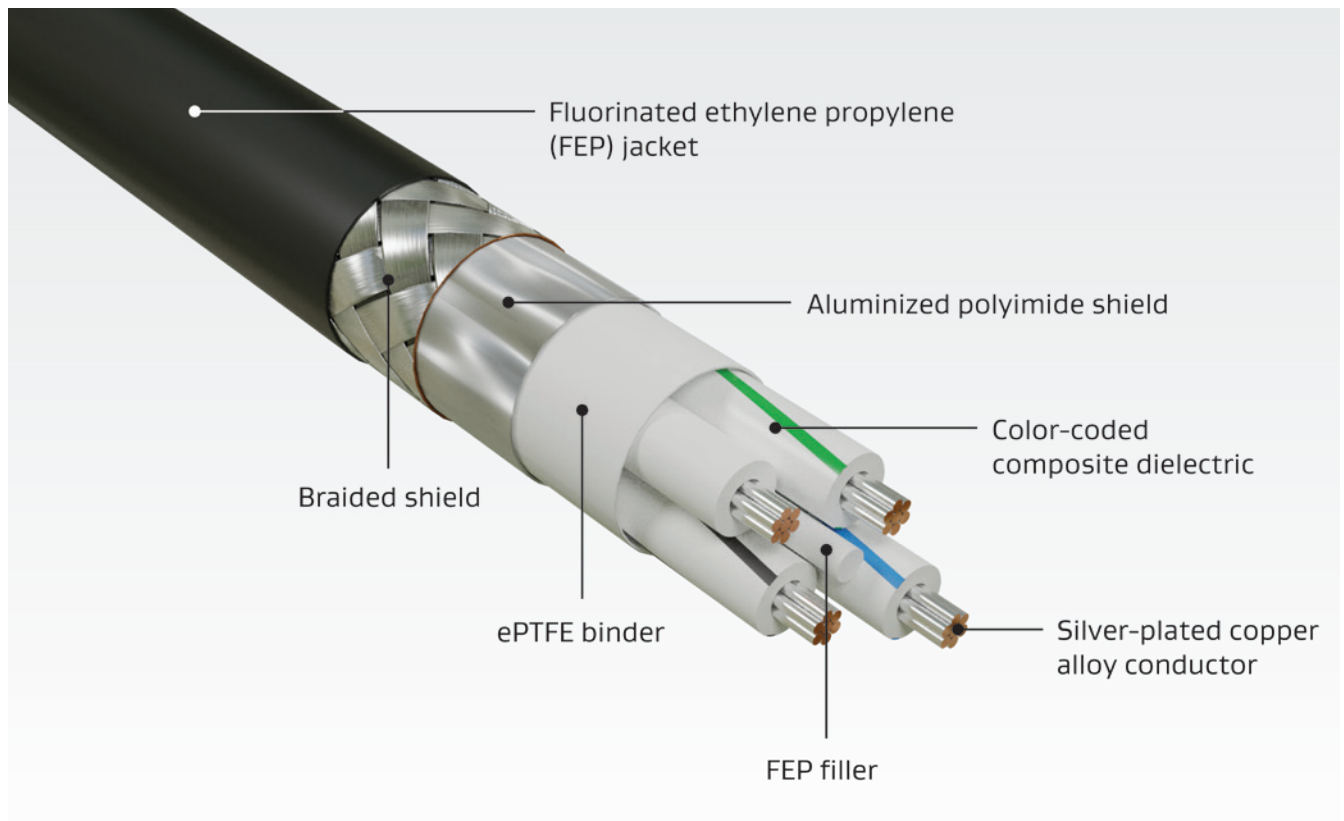
Figure 30: Tough Quadrx Construction
